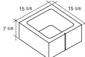
16x8x16 Vertical Score 1-Side
