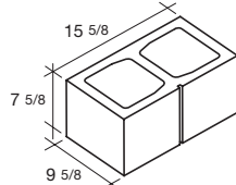
10x8x16 Vertical Score 1-Side
