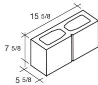
6x8x16 Vertical Score 1-Side
