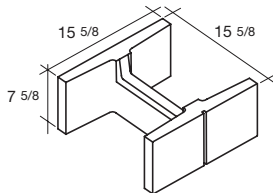
16x8x16 Double Open End Vertical Score 1-Side
