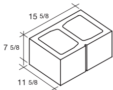
12x8x16 Vertical Score 1-Side
