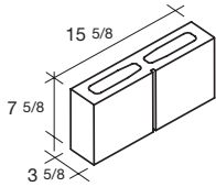
4x8x16 Vertical Score 1-Side
