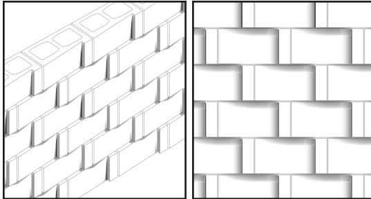
Spade Block Running Bond
