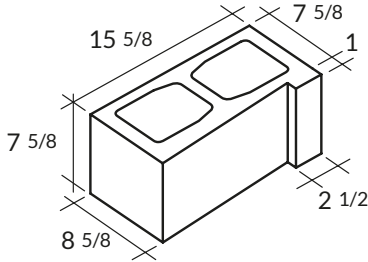
8x8x16 Spade Block
