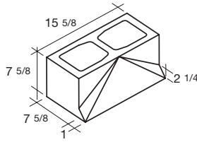
8x8x16 Shadow Block
