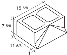
12x8x16 Shadow Block
