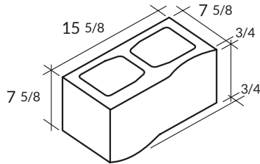
8x8x16 Ripple Block
