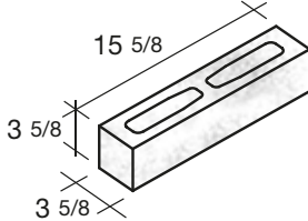
4x4x16 Standard Quik-Brik® (for anchored use)
