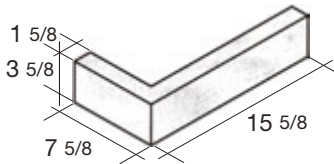
8x4x16 L-Corner Quik-Brik® Veneer (for adhered use in lightweight)
