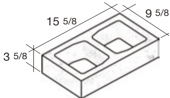
10x4x16 Quik-Brik®
