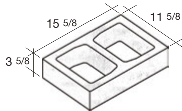
12x4x16 Quik-Brik®
