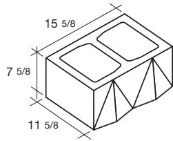
12x8x16 Hi-Lite Mark II
