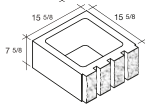
16x8x16 Ring 4-Score Split 1-Side
