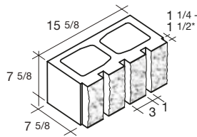
8x8x16 4-Score Split 1-Side
