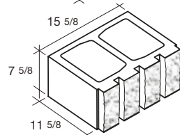
12x8x16 4-Score Split 1-Side
