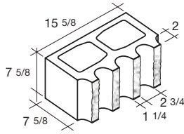
8x8x16 4-Flute Split 1-Side
