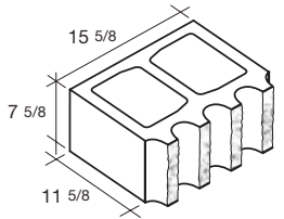
12x8x16 4-Flute Split 1-Side
