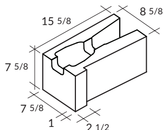
Spade Block Running Bond
