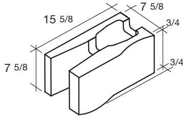
8x8x16 Ripple Block Open End Bond Beam
