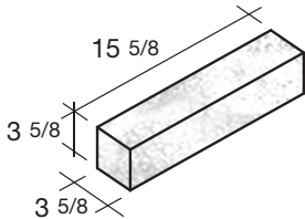
4x4x16 Solid Quik-Brik® Veneer (for anchored use)
