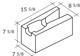
Facet Running Bond
