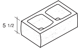
10x6x16 Standard
